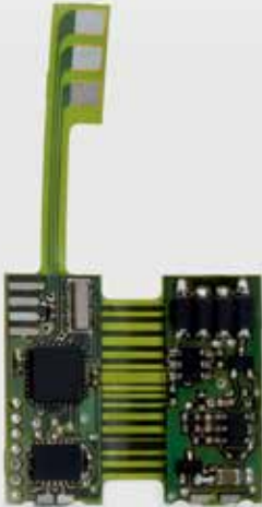
Drive electronics for lengthening human limbs (implant)
